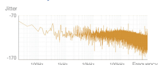
Audio clock jitter of conventional modules
