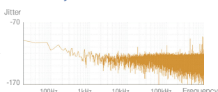
Audio clock jitter of the new module
