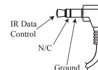
Figure 09– IR 3.5mm connector
